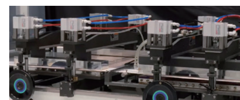
Straight sealing station
